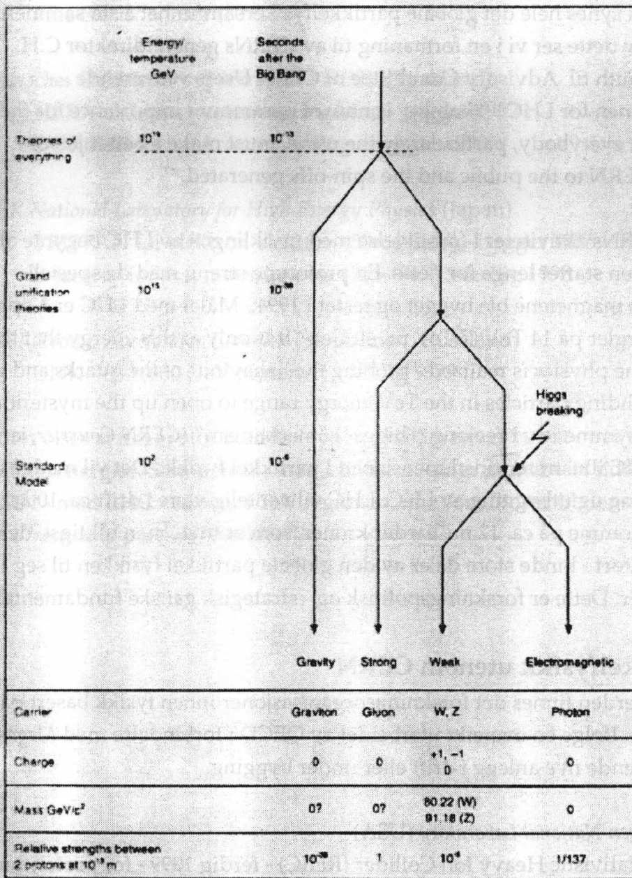
Figure 9. Temporal evolution of the Universe from the Big Bang
