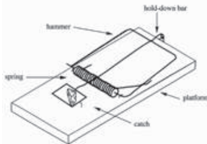
U.S.Patent: 1167493, 1916. Mousetrap
